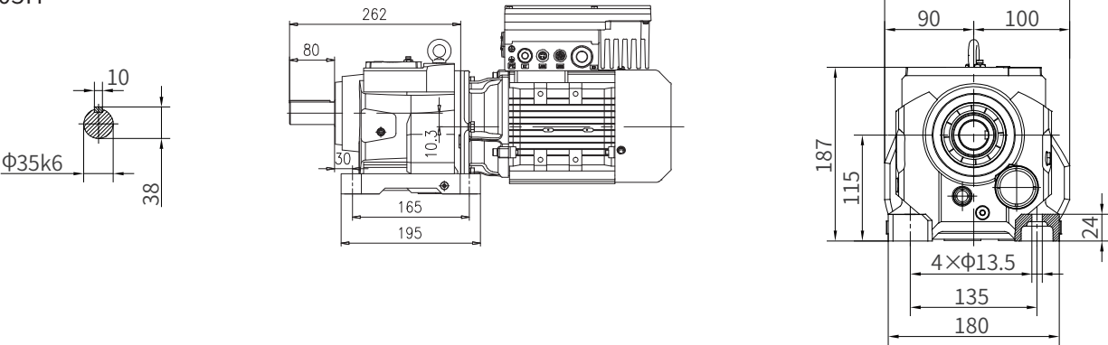
Horizontal foot-mounted
