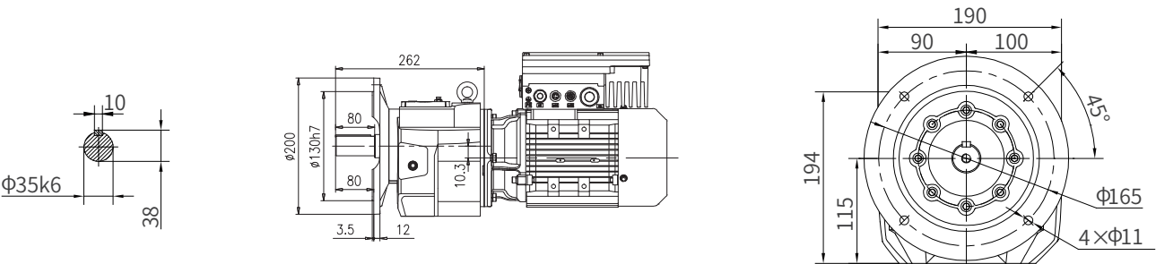
Flange-mounted
